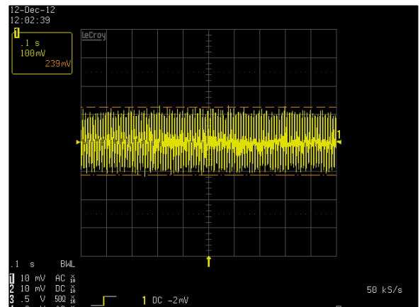
Figure 32: LCM300Q Ripple and Noise Measurement V_{in} = 90V_{ac} Load: I_O = 12.5A (24V), I_{SB} = 2A (5V) Ch 1: V_O
