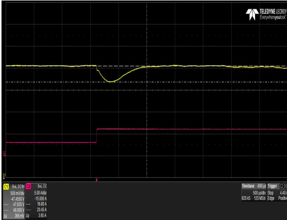
Figure 51: LCM300W Transient Response - Vo Deviation 50% to 100% load change 1A/µs slew rate Vin = 230Vac Ch 1: Vo Ch 2: Io
