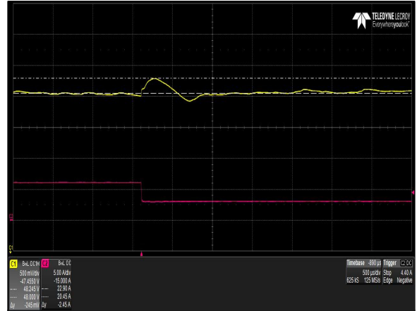
Figure 52: LCM300W Transient Response - Vo Deviation 100% to 50% load change 1A/µs slew rate Vin = 230Vac Ch 1: Vo Ch 2: Io
