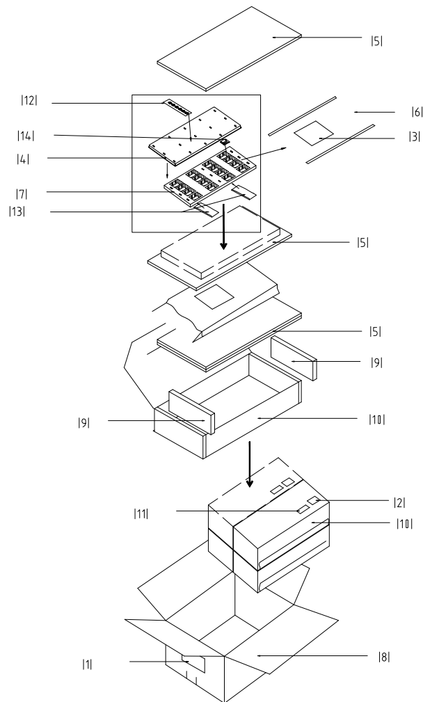
Figure 24: Package disassembly
