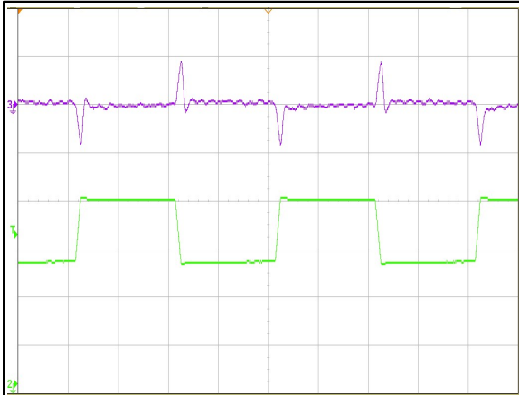
Figure 7: ADO300-48S12 Transient Response (500uS/div) 50%~75%~50% load change, 0.1A/uS slew rate Ch 3: Vo (200mV/div) Ch 2: Io (5A/div)
