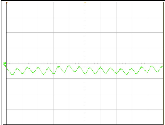
Figure 1: ADO300-48S12 Input Reflected Ripple Current Waveform Ch 2: Iin (5uS/div, 20mA/div)
