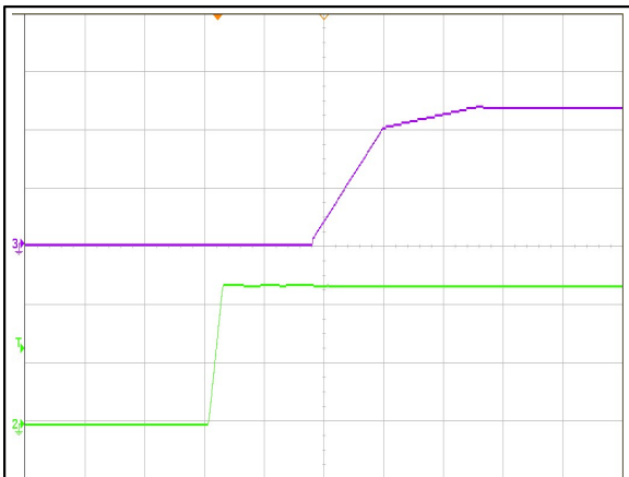
Figure 3: ADO300-48S12 Output Voltage Startup Characteristic (20mS/div) Ch 3: Vo (5V/div) Ch 2: Vin (20V/div)
