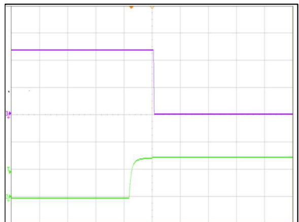
Figure 6: ADO300-48S12 Remote OFF Waveform (200mS/div) Ch 3: Vo (5V/div) Ch 2: Remote ON (2V/div)
