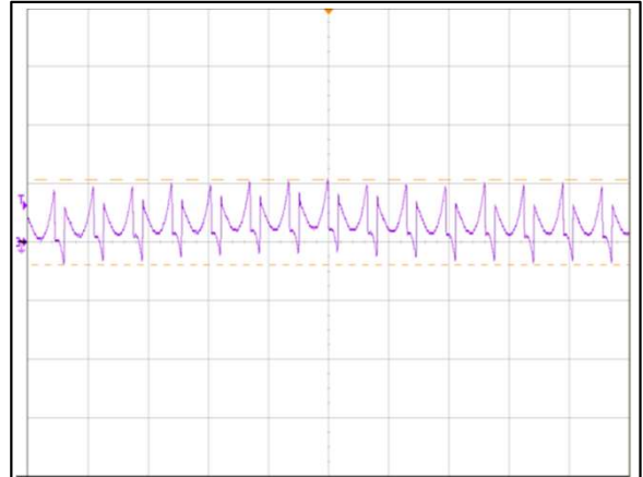
Figure 2: ADO300-48S12 Ripple and Noise Measurement Ch 3: Vo (5uS/div, 20mV/div)
