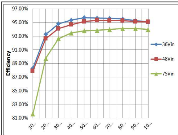
Figure 9: ADO300-48S12 Efficiency vs. output current, Ta=25oC, Vo=11.9V Loading: Io = 10% increment to 26A
