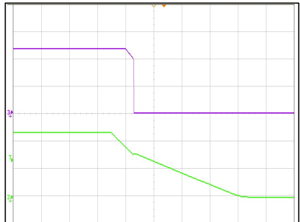
Figure 4: ADO300-48S12 Turn Off Characteristic (100mS/div) Ch 3: Vo (5V/div) Ch 2: Vin (20V/div)
