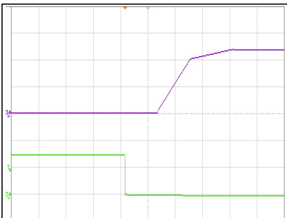
Figure 5: ADO300-48S12 Remote ON Waveform (20mS/div) Ch 3: Vo (5V/div) Ch 2: Remote ON (2V/div)
